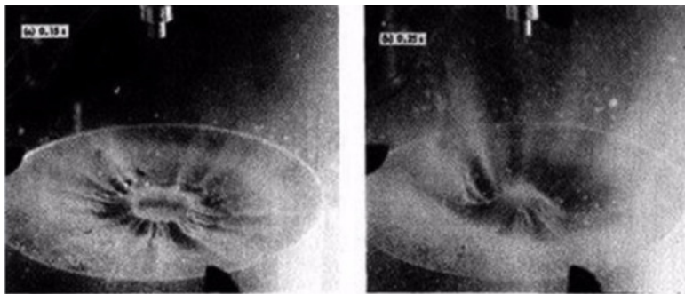
Fig. 10. Movie frames of jet firing in test A2a
