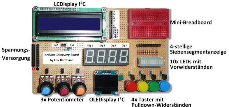
Abb. 1: Das Arduino-Discoveryboard
