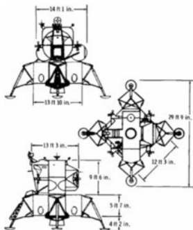
Figure 3. - Basic LM dimensions.
